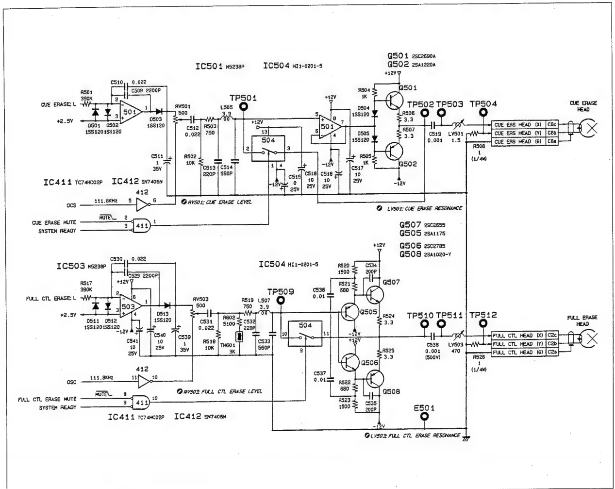
Fig. 2-8-1. Erase Amplifier (AE-05 Board)
